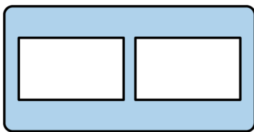
Monolithic architectures
