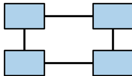
Distributed architectures
