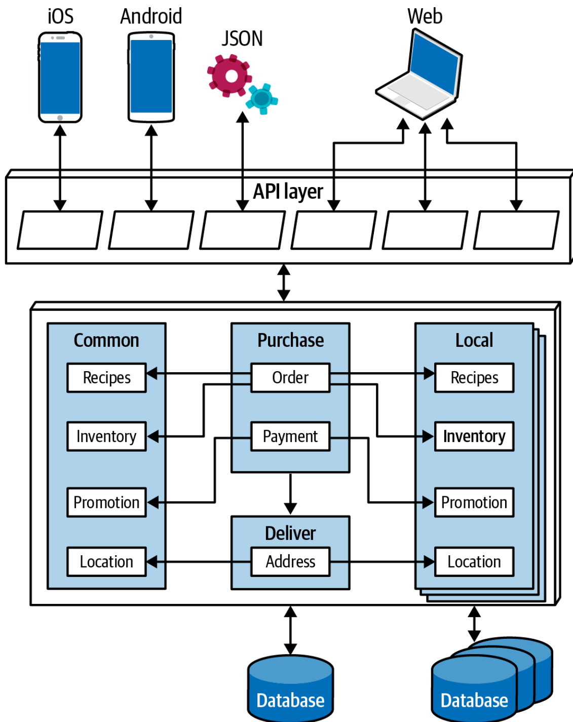
Figure 19-4. A microkernel implementation of Silicon Sandwiches
